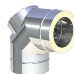
Inspection elbow 87° with inspection door for wet opera- tion mode (up to 250°C/H1)
