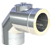
Coupling elbow 87°, 200°C/P1 with inspection, suitable for DWKL07
