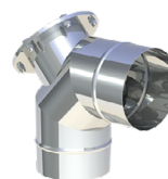
Elbow 90° with inspection door, wet operation mode (up to 250°C/HI)
